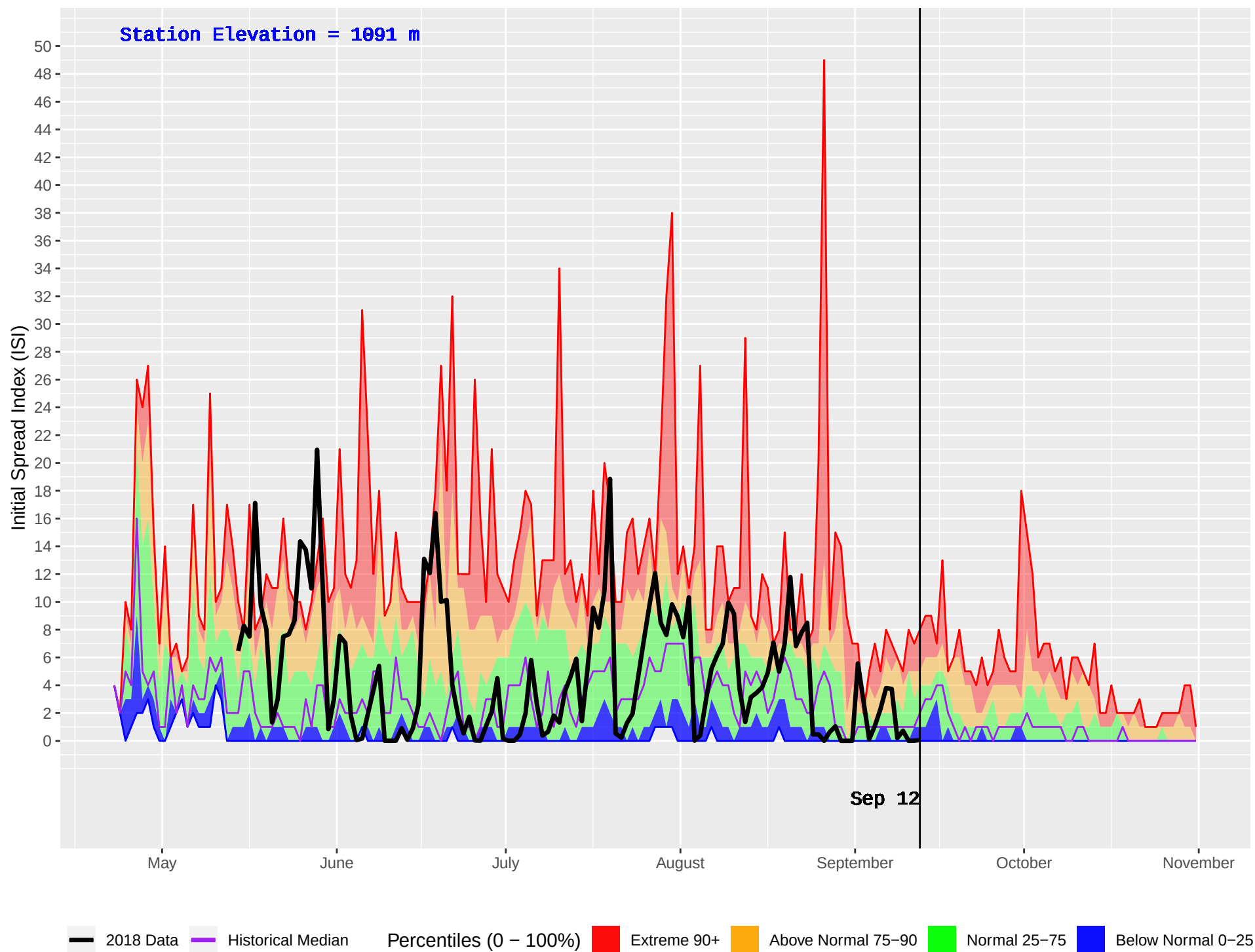
BIG MOUTH 2 (868) : Historical (2004–2016) and Current (2018) Daily Initial Spread Index (ISI)
