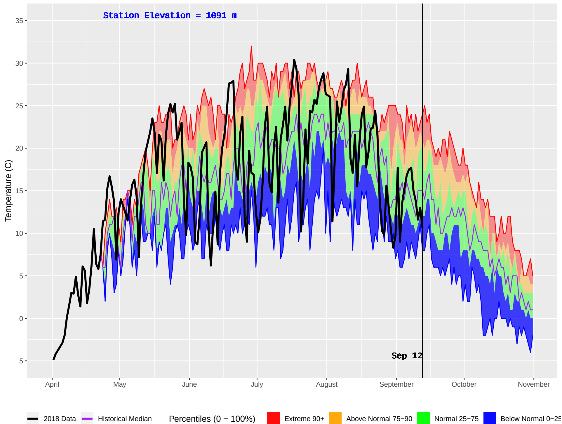
BIG MOUTH 2 (868) : Historical (2004–2016) and Current (2018) Daily Temperature
